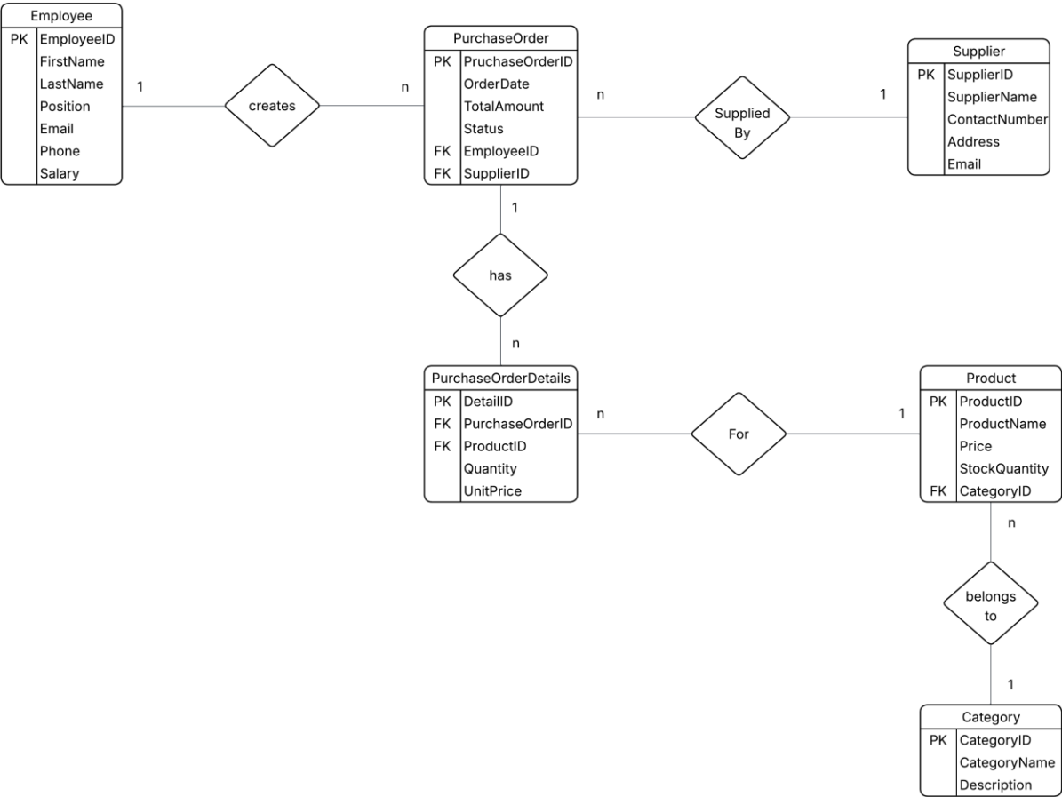
Figure 3: ER diagram of System
